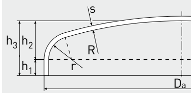
PLATE-TYPE HEAD
