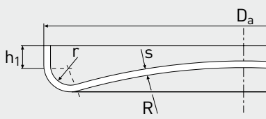
INSPECTION COVERS
