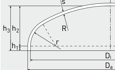
ELLIPTICAL HEAD
