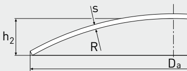
DIFFUSER HEAD
