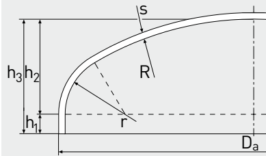
SEMI-ELLIPTICAL HEAD
