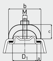
HEAD- AND MANHOLE with warm pressed cover
