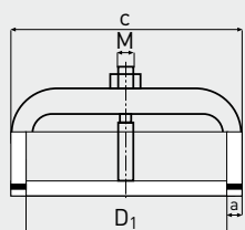
HEAD- AND MANHOLE with flat machined cover
