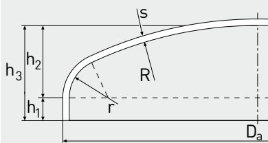
CONVEX DISC
