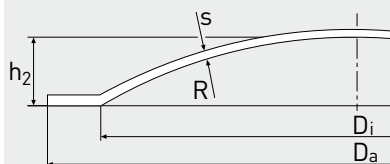
PLATE-TYPE HEAD
