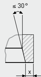
FORM BI TAPERING INSIDE
