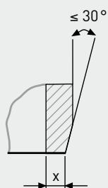
FORM BA TAPERING OUTSIDE
