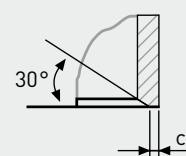
FORM BI TAPERING INSIDE
