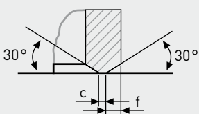
FORM DY DOUBLE Y
